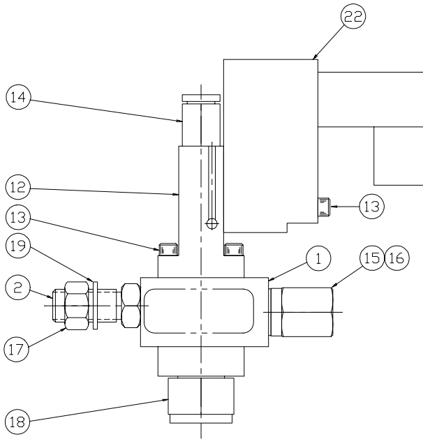
369 valve shown with M16 nozzle adapter
