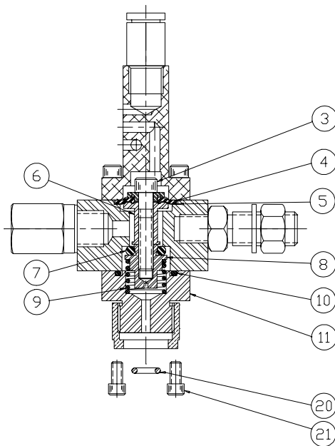
Items 20 and 21 used only with block adapter assemblies
